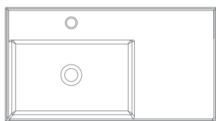
Art. 5115 - 80 x 44 x h14 cm TEOREMA 2.0 80 SHELF DX®
