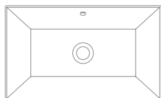
Art. 5131 - 60 x 36 x h5 cm / total 17 cm TEOREMA 2.0 60x36
