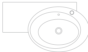
Art. 2012 - 87 x 52 x h13,5 cm WISH SHELF SX
