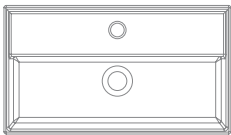
Art. 5002 - 60 x 34 x h14 cm TEOREMA 60X35R
