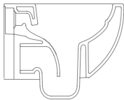
5524/CL - 45 x 35 MOON CLEAN FLUSH HUNG WC Wc Sospeso - Wall-mounted WC - Cuvette suspendue Hänge-WC - Inodoro Suspendido - Унитаз подвесной
