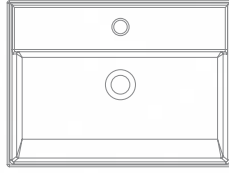
Art. 5109 - 60 x 44 x h7 cm / total 17 cm TEOREMA 2.0 60A BUILT-IN
