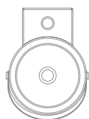
Art. 8802 - 30 x 40 x h22,5 cm BUCKET 30R
