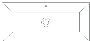
Art. 5132 - 80 x 36 x h5 cm / total 17 cm TEOREMA 2.0 80x36
