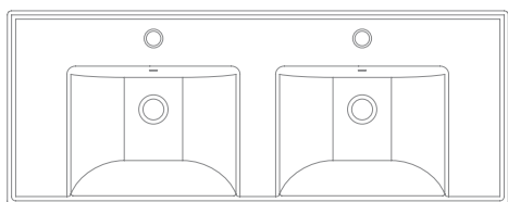
Art. 3006 - 122 x 47 x x h5 cm / total 16 cm ML 120 x 47
