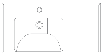
Art. 3008 - 92 x 47 x h5 cm / total 18 cm ML 90 x 47 SHELF DX
