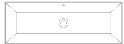
Art. 5137 - 100 x 36 x h0 cm / total 17 cm TEOREMA 2.0 100x36S
