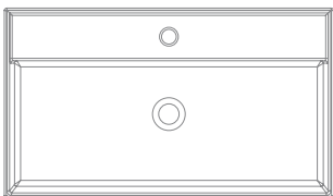
Art. 5110 - 80 x 46 x h14.5 cm TEOREMA 2.0 80R
