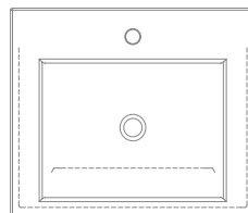
Art. 8007/A - 61 x 51 x h8,5 cm / total 16 cm SQUARE 60A
