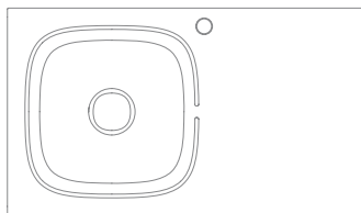
Art. 1890 - 86 x 50 x h7 cm / total 23 cm UP SHELF DX
