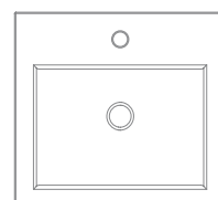
Art. 8025/B - 51 x 46 x h16 cm SQUARE 50B
