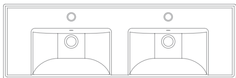
Art. 3003 - 122 x 40 x h5 cm / total 16 cm ML 120 x 40
