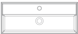
Art. 5003 - 80 x 34 x h14 cm TEOREMA 80X35R
