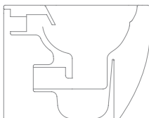
Art. 5138/CL - 55 x 36 x h42 cm TEOREMA 2.0 CLEAN FLUSH WC
