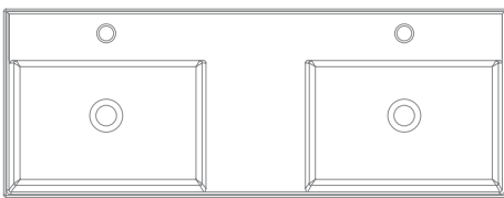
Art. 5143 - 121.5 x 46 x h14 cm TEOREMA 2.0 121 x 46
