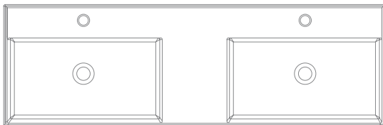
Art. 5116 - 141.5 x 45.5 x h14 cm TEOREMA 2.0 141 x 46
